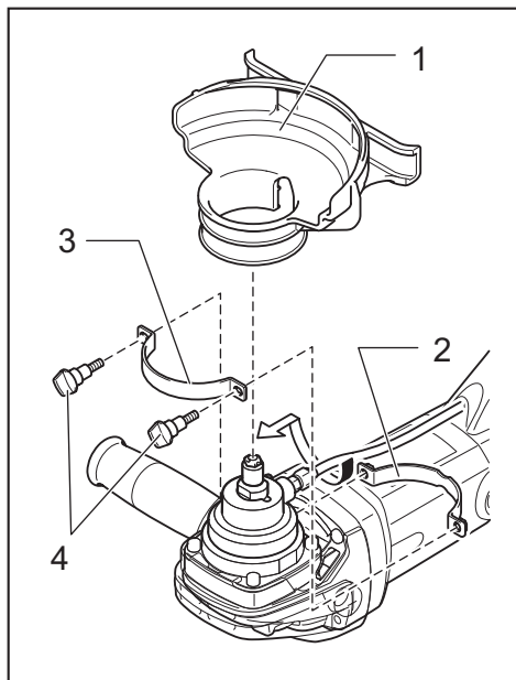
► 1. 125mm dust cover 2. Dust cover band A 3. Dust cover band B 4. Screws
