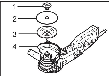
► 1. Lock nut 2. Abrasive disc 3. Rubber pad 4. 125 mm dust cover
